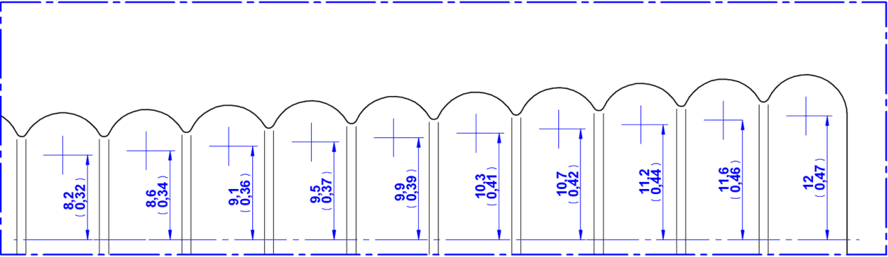
DETAIL A
